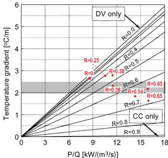
Figure 9. Design diagram developed by Tan et al. (1998). In this graph R is equal to \eta and P/Q is CC/V_{air} . Published 2012 | Page 9 of 11
